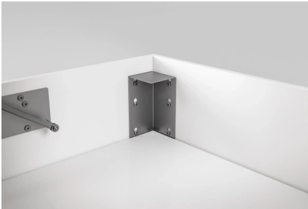
Angle blocks Elements to join the bed frame with a quick, solid and neat result. The four corner blocks support the entire bed frame.
