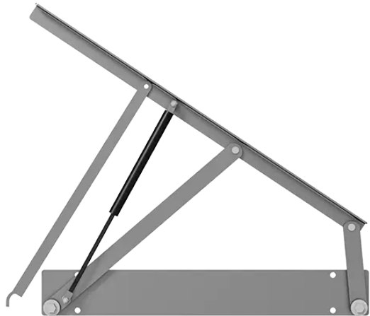
Gas Spring
